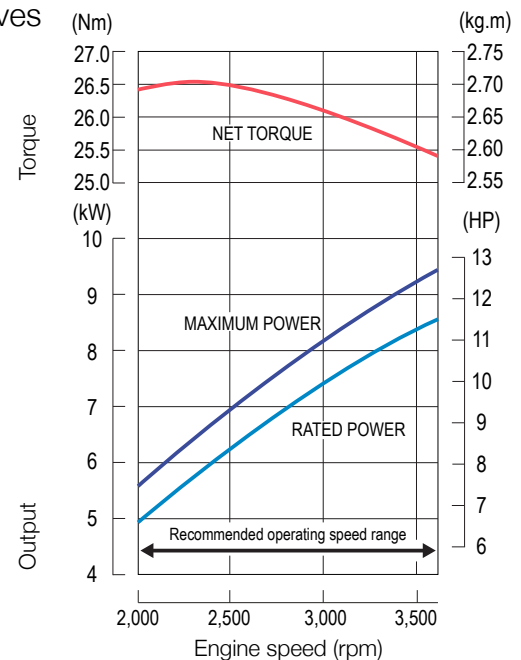
Power Curves
